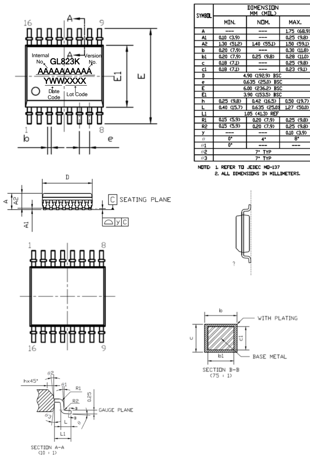
Figure 6.1 – SSOP 16 Pin Package (150 mil)
